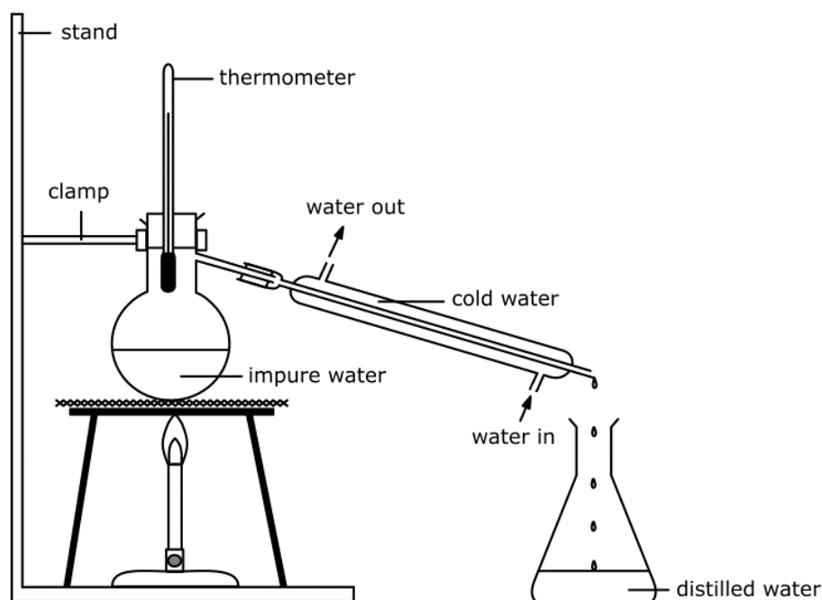
Distillation
